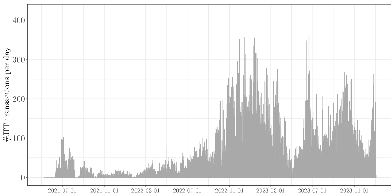
Figure 6: JIT Liquidity Transactions. This figure shows a timeseries of the number of ‘just-in-time’ liquidity transactions per day. The sample period is from the launch of Uniswap V3 (May 2021) to December 31, 2023.
