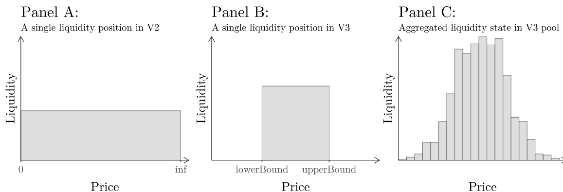
Figure 2: “Liquidity state in Uniswap V2 and V3” adapted from Adams et al. (2021). This figure exemplifies the liquidity states in Uniswap V2 and V3. Panel A shows the liquidity state in a Uniswap V2 pool that provides liquidity across the whole price range. Panel B shows the liquidity distribution of a single, concentrated liquidity position in Uniswap V3 that distributes its liquidity in a price range between a lower bound and an upper bound. Panel C depicts the aggregated liquidity state of multiple liquidity positions in a Uniswap V3 liquidity pool.
