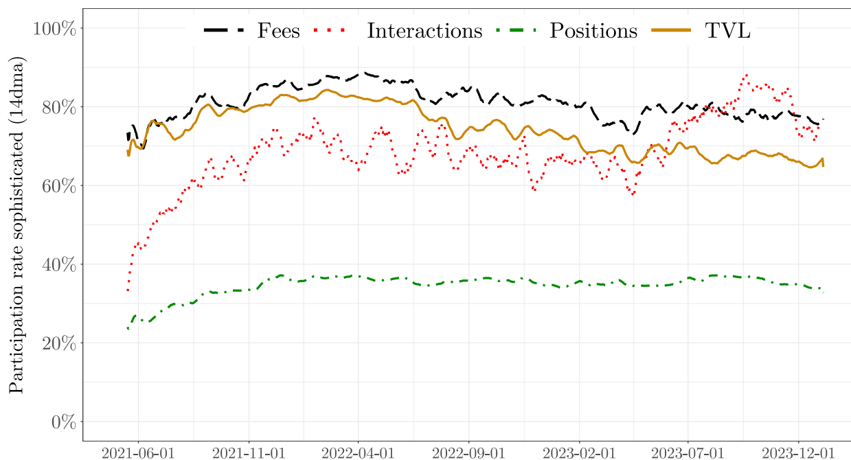
Figure 7: Participation of sophisticated LPs at the protocol level. This figure shows the participation rate of sophisticated market participants across multiple dimensions. Daily pool values are aggregated using a 14 days moving average. Fees is the USD of accrued fees, Interactions is the number of liquidity related transactions, positions is the proportion of fee-collecting liquidity positions and TVL is the total-value locked in USD.
