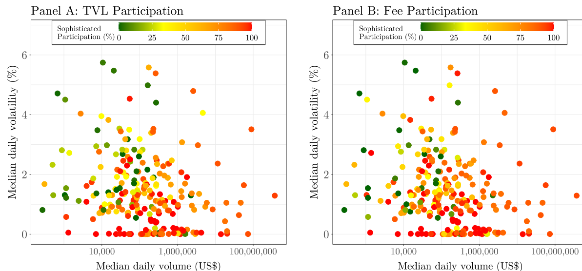
Figure 8: Sophisticated participation at the liquidity pool level. This figure illustrates the dominance of sophisticated market participants in terms of total-value locked (Panel A) and accrued fees (Panel B). Each dot represents one of the 250 liquidity pools and relates the median daily volatility expressed as a percentage with the median USD daily trading volume of a pool. The x-axis is log-scaled. The color represents the sophisticated participation rate, with green indicating low dominance of sophisticated liquidity providers in a liquidity pool and red indicating high sophisticated dominance.
