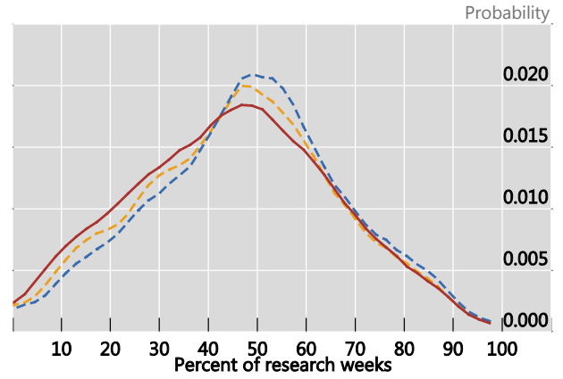
Density function
