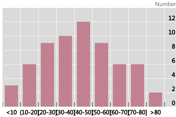
Histogram
