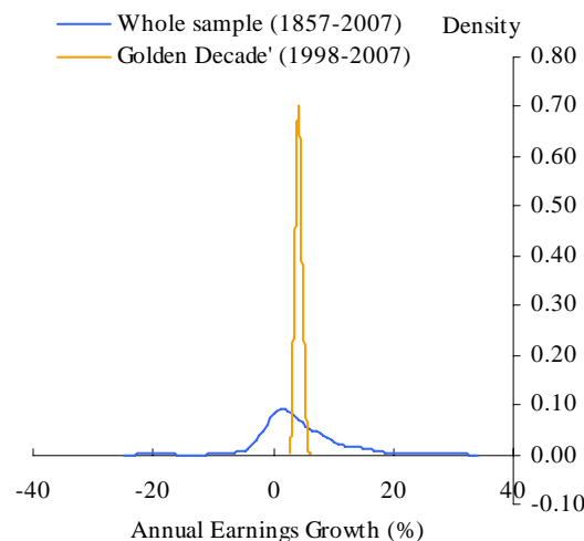
Chart 4: Probability density estimates for Annual Earnings Growth
