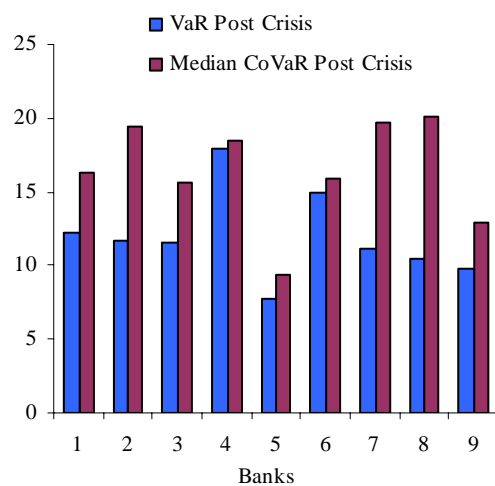
Chart 12: VaR vs CoVaR for a selection of major UK banks, post crisis
