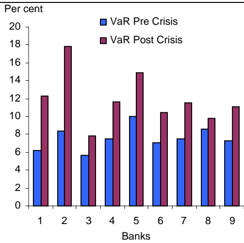
Chart 9: 90th Percentile VaR for a selection of major UK banks, pre and post crisis
