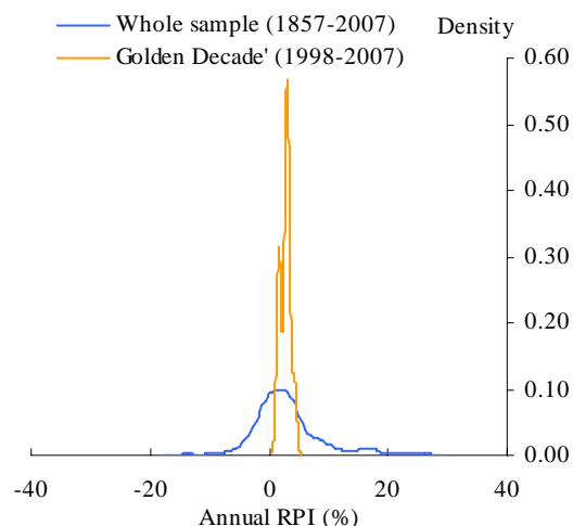
Chart 2: Probability density estimates for UK RPI
