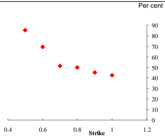
Chart 10: Percentage under-valuation of a put option on UK equities during the Golden Decade
